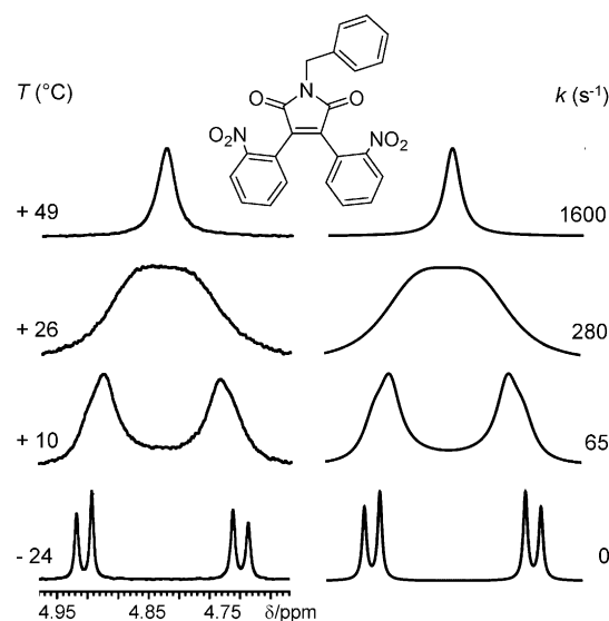
Figure 2. Variable-temperature 1 H NMR spectra of 1 (600 MHz in CDCl 3 ). Left: experimental spectra. Right: simulated spectra with the relative rate constants.
