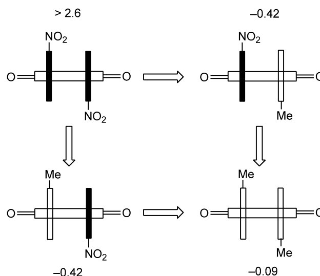
Scheme 2. DMC cycle for compounds 1–3 . The indicated values (in \text{kcal mol}^{-1} ) are the energy differences ( \Delta G^{\circ} ) between the anti and syn conformers as measured by NMR spectroscopy at -40^{\circ}\text{C} . Negative values indicate that the syn conformation is more stable than the anti conformation.
