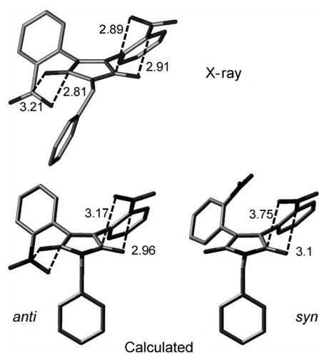
Figure 1. Top: X-ray crystal structure of compound 1. Bottom: calculated structures of the anti and syn conformers at the \omega B97XD/6-311++G(2d,p) level. Distances in Å.
